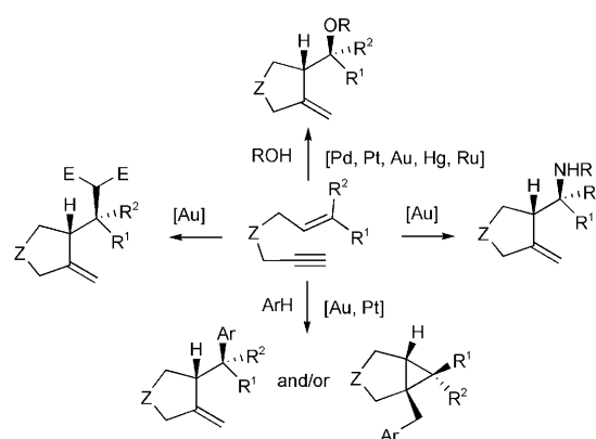
Scheme 1. Metal-catalyzed cycloisomerization of 1,6-enynes in the presence of an external nucleophile.
