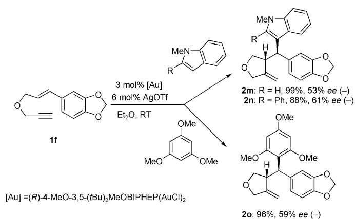
Scheme 2. Asymmetric Au I -catalyzed cycloisomerization of oxygen-tethered 1,6-enynes.
