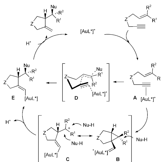
Scheme 4. Mechanism rationale.
