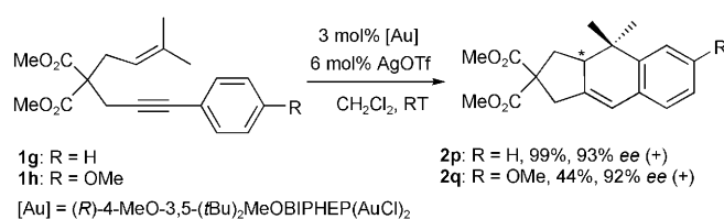
Scheme 3. Asymmetric intramolecular Au I -catalyzed cycloisomerization of 1,6-enynes.
